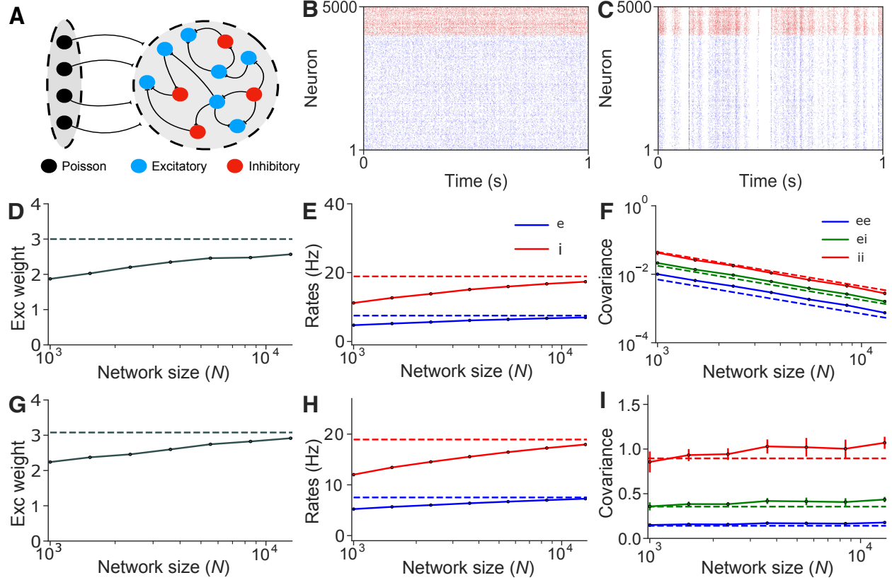
Figure 3.1.4: A plastic, balanced network in asynchronous and correlated regimes. A: A recurrent network of excitatory, E , and inhibitory, I , neurons is driven by an external feedforward layer, X , of correlated Poisson neurons. B: Raster plot of all neurons in a network of N = 5000 neurons in an asynchronous state. E cells in blue, I neurons in red. C: Same as ( B ), but in a correlated state. D: Mean steady state EE synaptic weight, j_{ee} , in an asynchronous state. E: Mean E and I firing rates for different network sizes, N , in an asynchronous state. F: Mean EE , II and EI spike count covariances in an asynchronous state. G–I: Same as ( D–F ) but for a network in a correlated state. Solid lines represent simulations, and dashed lines are values obtained using Eqs. (2.26, 2.105, 3.6). All empirical results were averaged over 10 realizations. In the asynchronous state c_x = 0 , and in the correlated state c_x = 0.1 . Unless otherwise stated, colors carry the same meaning in all figures. Figure adapted from Akil et al. [5].
